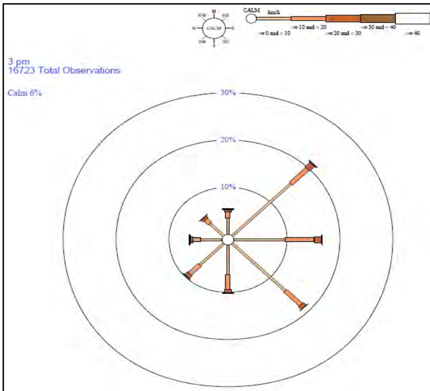
Figure 6-3 Annual Average 3 pm Wind Rose – Barcaldine Post Office (1962–2010)
